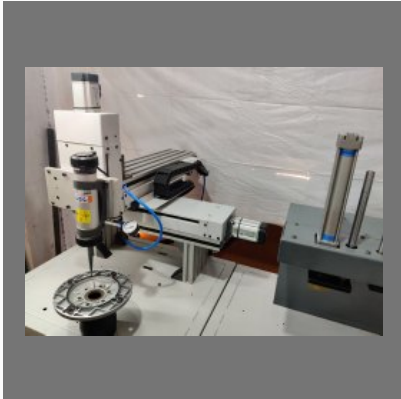
Automatic Gasket Sealant Dispensing Robotic System
