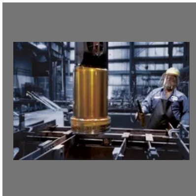
Chrome Coating Service On Lead Roll
