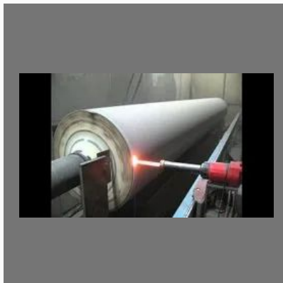
Tungsten Carbide Coating On Yankee Cylinder
