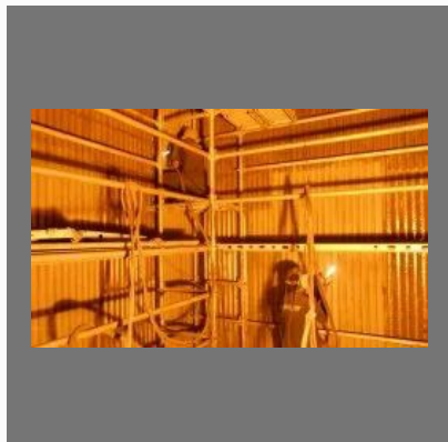
HVOF Thermal Spray Coating Service On Boiler Tube
