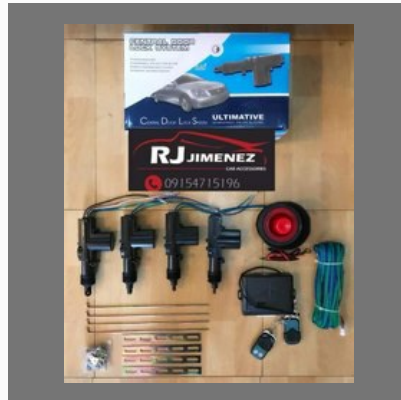
Alarm System
