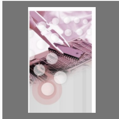
Software Prototyping
