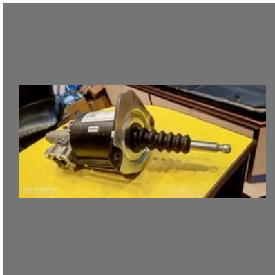
Clutch Booster 102mm Bharat Benz 2523
