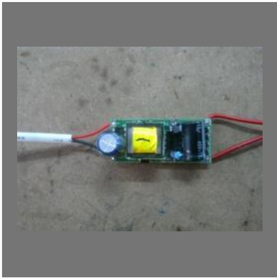
AC Input LED Drivers
