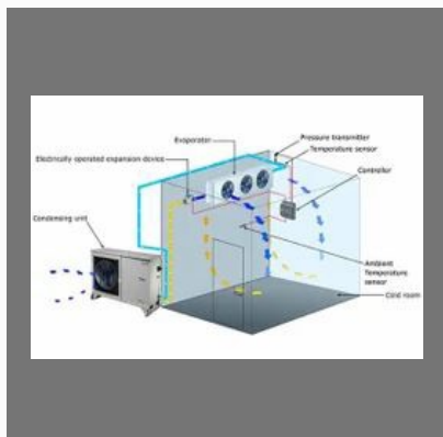
Cold Storage System
