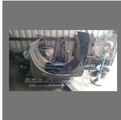
Voltas Forklift Paper Roll Clamp
