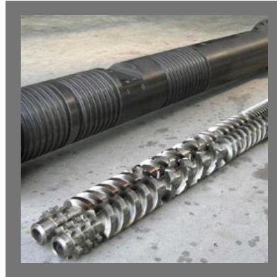
Screw Barrel
