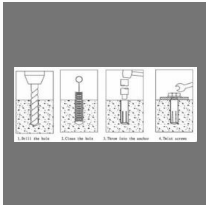
Drop In Anchor Or Bullet Fasteners M20
