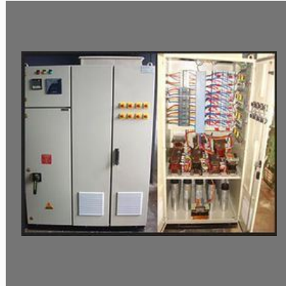
APFC Panels
