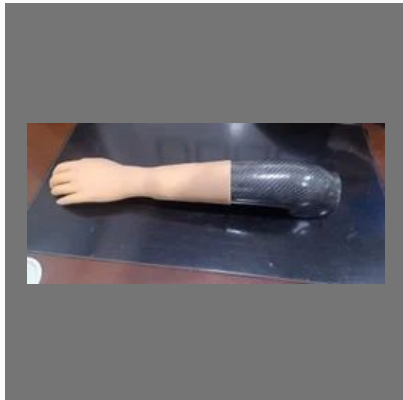
Below Elbow Prosthesis
