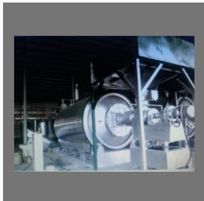
Pyrolysis Plant ,Batch To Continuous Tire Pyrolysis Plants Conversion System Batch Type
