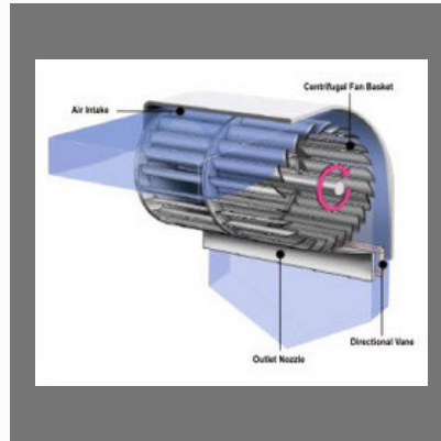
Air Curtains (02)
