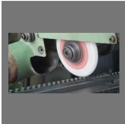
Broach Resharpener
