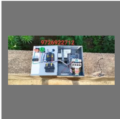
DOL Type Submersible Pump Control
