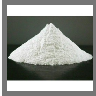
Sodium Carbonate
