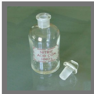
Nitric Acid
