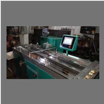
Automatic Programmable Notepad Slip Pad Wire Stitching Machine
