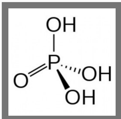
Ortho-Phosphoric Acid 85%
