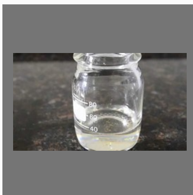
Methyl Benzoate
