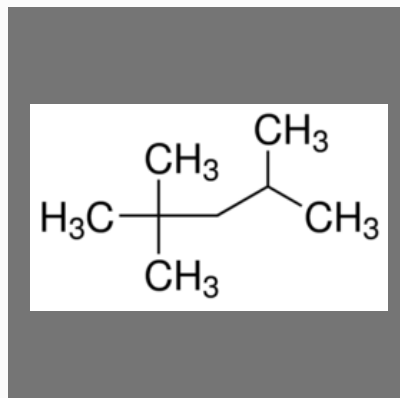
2,2,4-Trimethylpentane
