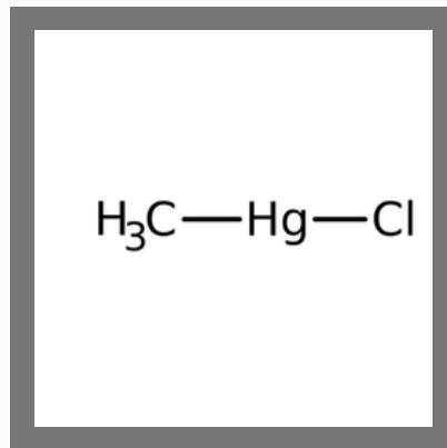
Methylmercury(Ii) Chloride
