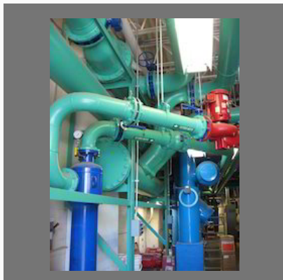
Water Chilling Plant
