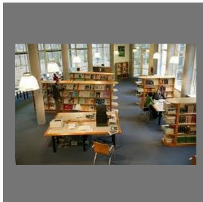
Library Management
