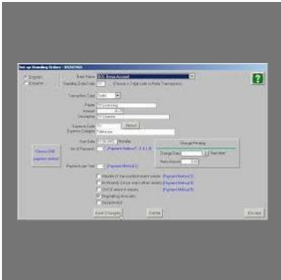
Banking Software
