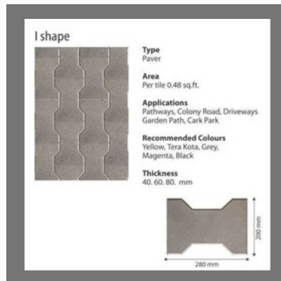
Paver Block - I-Shape
