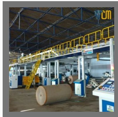
Automatic Board Making 3 / 5 Ply Plant - STD Board Line
