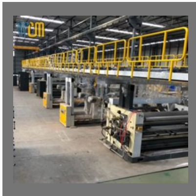
Automatic 3 / 5 Ply Plant - XPS Line
