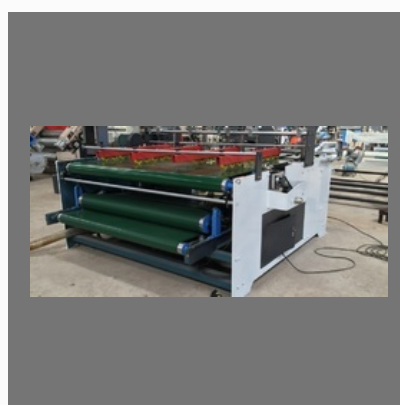
Corrugated Box Flap Pasting Machine
