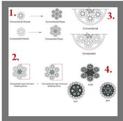
Power Form Steel Wire Rope
