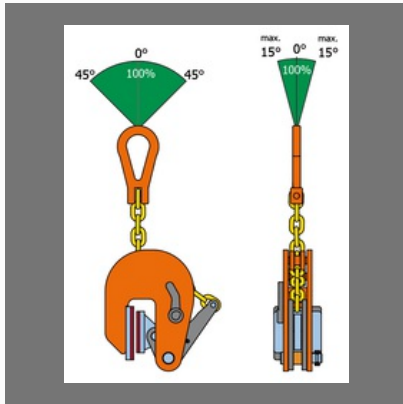
Pewag Lifting Clamp for SS Plates Non- Marking
