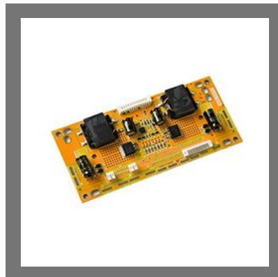
Gold-99E LED Backlight Inverter Board 21-65 Inch LED Backlight Driver Board Input Volt - 24V
