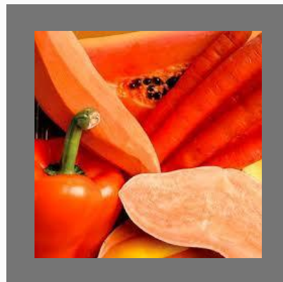
Beta-Carotene
