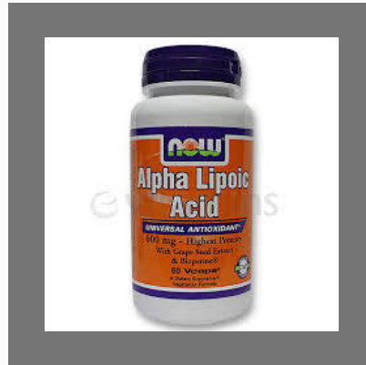
Alpha-Lipoic Acid
