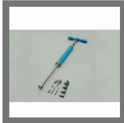
Proctor Penetrometers Proctor Needle Spring Type
