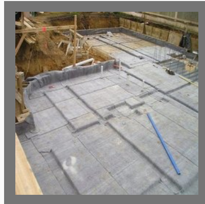
Basement Waterproofing By HDPE Membrane
