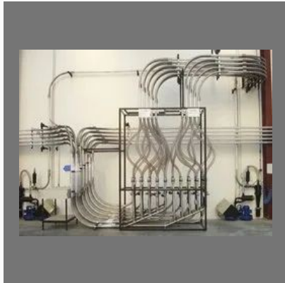
Vacuum Pneumatic Conveying Systems
