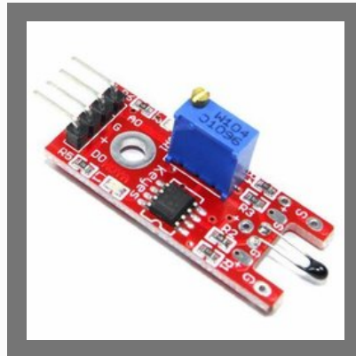
ARDUINO Digital Temperature Sensor Module
