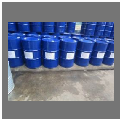
Benzyl Salicylate .
