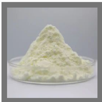
Benzophenone Powder
