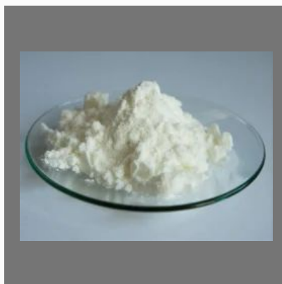
Cinnamic Acid
