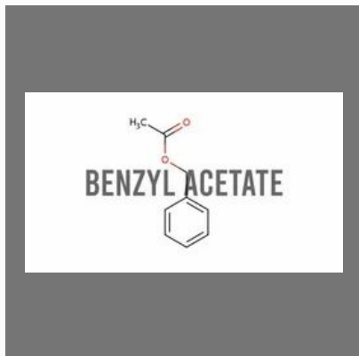
BENZYL ACETATE
