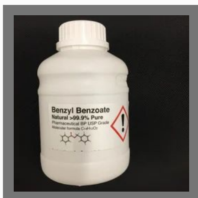
Benzyl Benzoate
