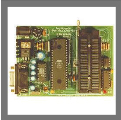
Device Programmer
