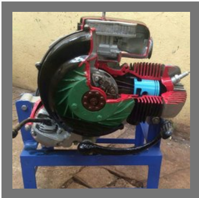
2 Stroke Petrol Engine Cut Section Model
