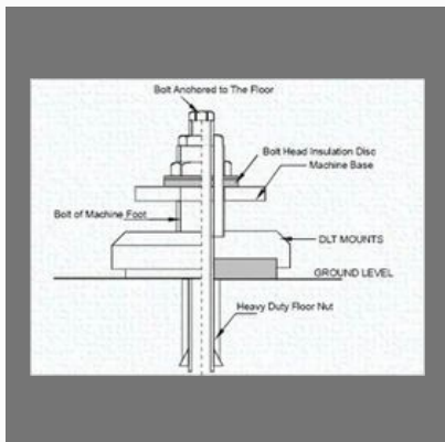
Screw Support Mounts
