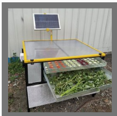
Solar Dryer With Fan
