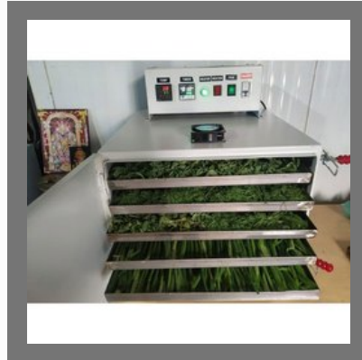
Vegetable Dehydrator
