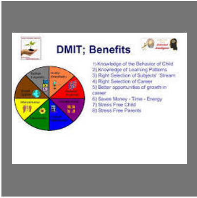
DMIT Software
