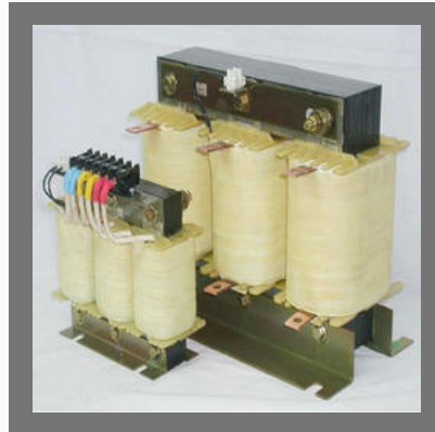
Detuned Capacitor
