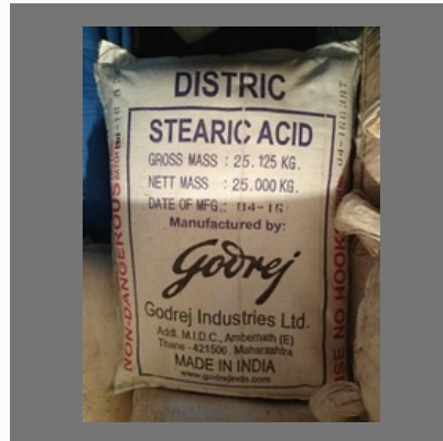
Stearic Acid
