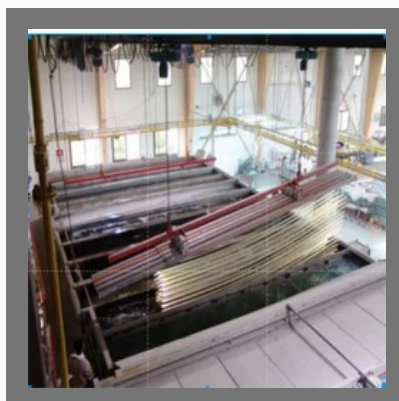
Anodizing Plant .
