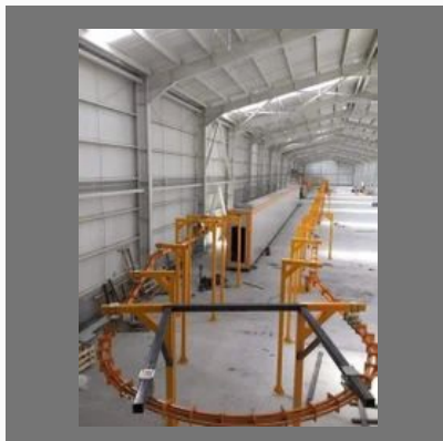
Four Wheel Overhead Conveyor
