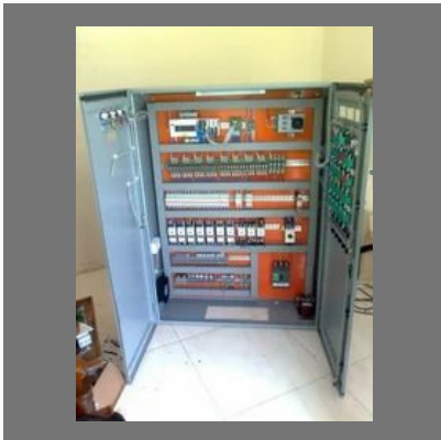
SCADA Automation Panel
