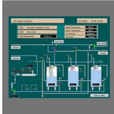
HMI Automation Panel
