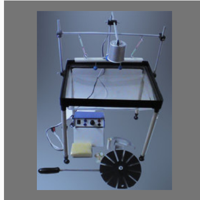
Ripple Tank Apparatus
