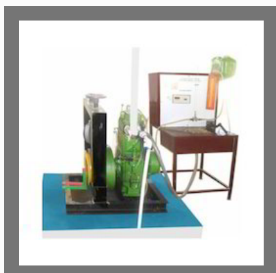
Single Cylinder 4 Stroke Diesel Engine with Mechanical Load
