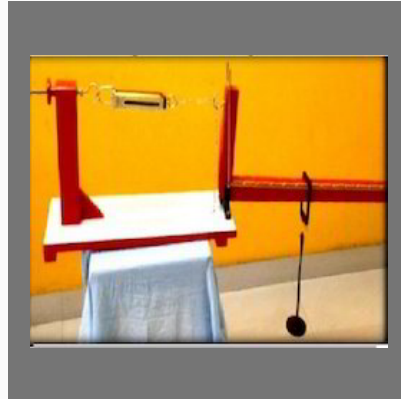
Bell Crank Lever
