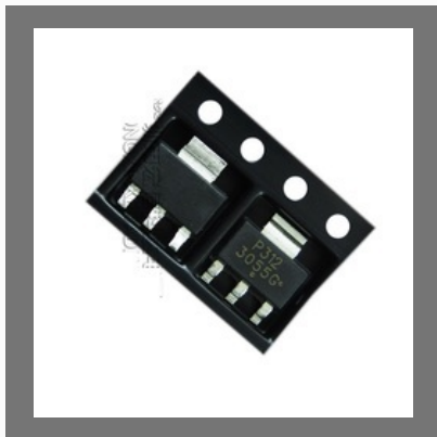
NTF3055 Power MOSFET 3.0 Amps, 60 Volts N Channel SOT223 SMD
