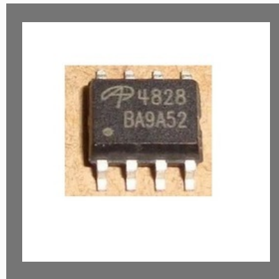
AO4828 DUAL N-Channel MOSFET 60V 4.5A SMD 8- SOIC
