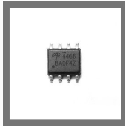
AO4466 MOSFET N-Channel 30V 10A SMD 8-SOIC SOP8
