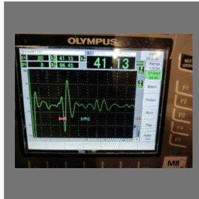
Composite Inspection
