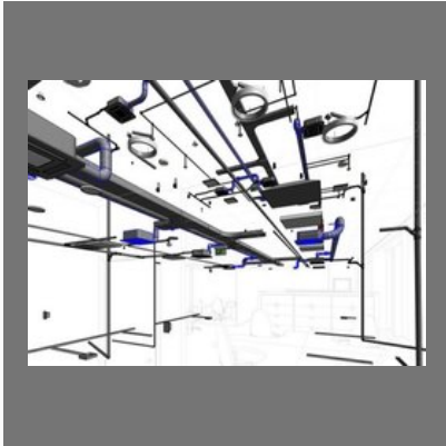
MEP BIM Modeling
