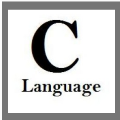
C Language
