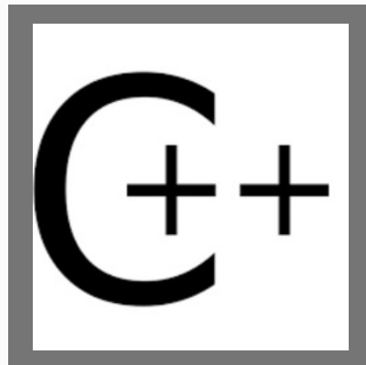
C++ Languages
