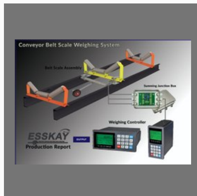
Dynamic Belt Weigher
