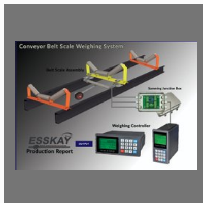
conveyor belt scale
