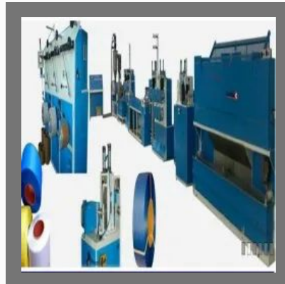
PP Box Strap Extrusion Line
