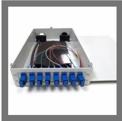
24 Port Liu Fully Loaded Patch Panel
