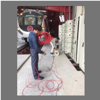
Fire Detection Tube Suppression System
